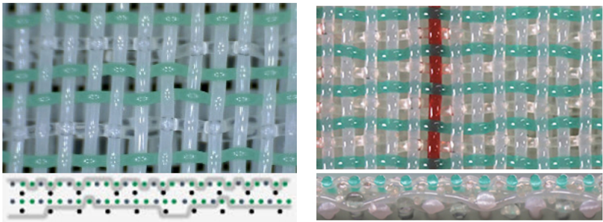
Triple Layer Forming Fabric
